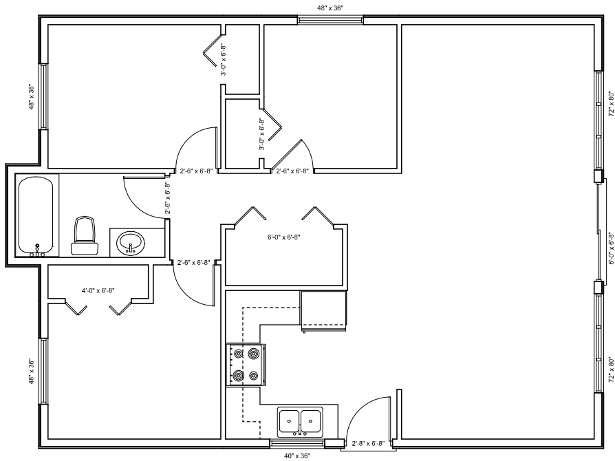
THE SOUTH RIDGE 896 SF. (36 wide x 24 long)
